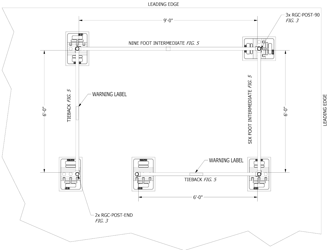
Figure 2 - Typical Layout
