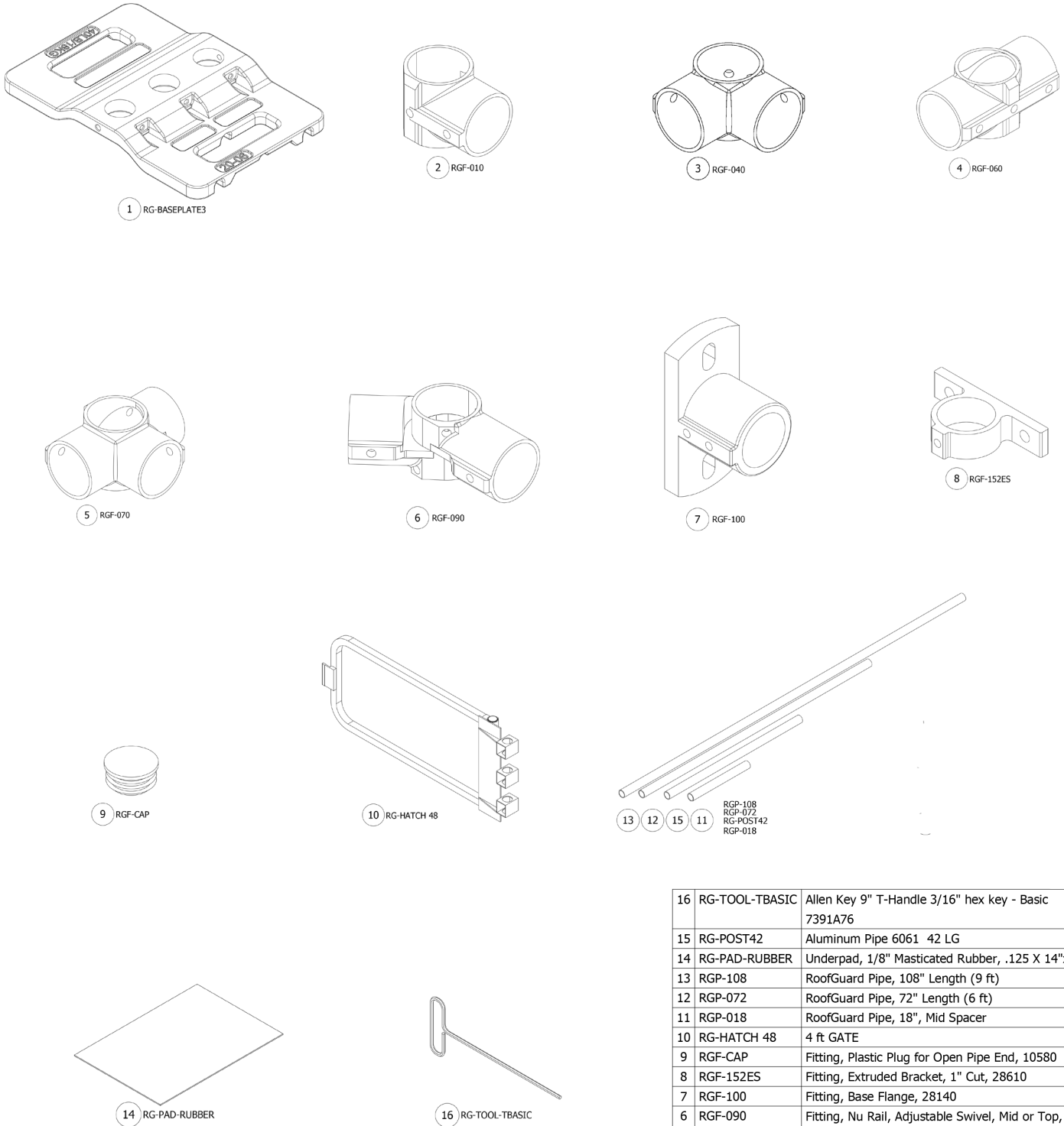
Figure 1 - Component Identification
