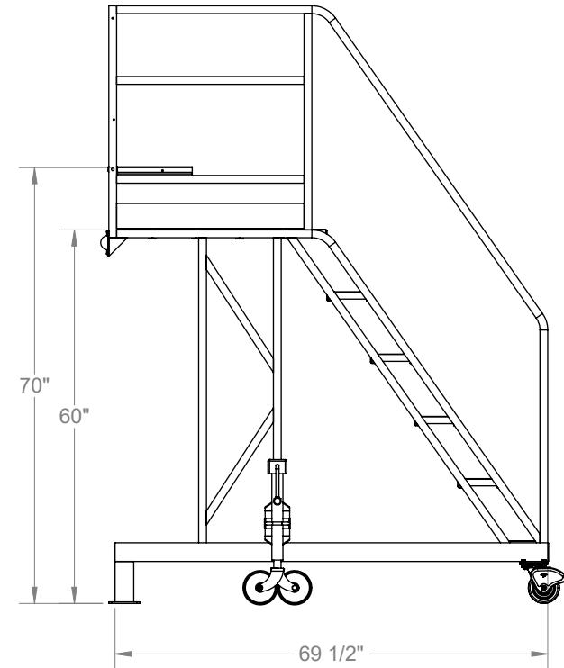
UPPER ACCESS STEP IN EXTENDED POSITION
