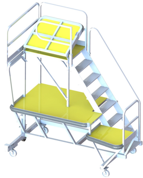
UPPER ACCESS PLATFORM IN FOLDED POSITION
