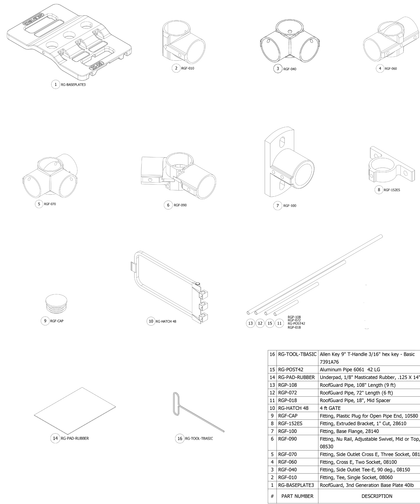
Figure 1 - Component Identification
