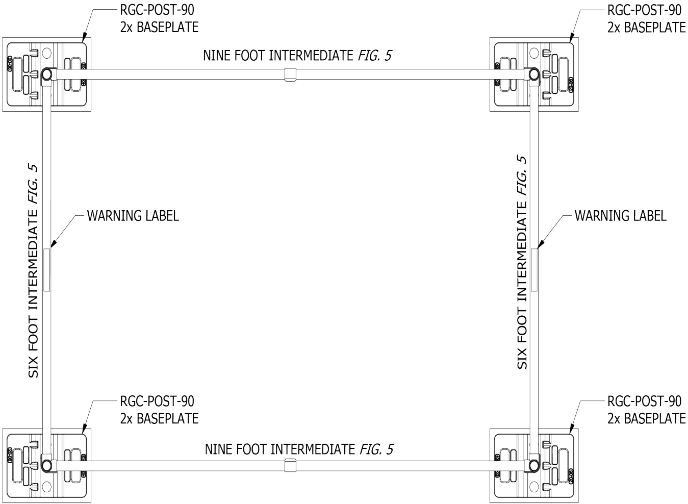
Figure 6 - Skylight Rails
